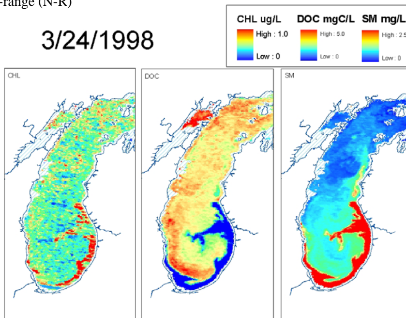
Figure 1. This figure presents the spatial distributions of chl, doc, and sm as they are retrieved from a SeaWiFS image taken on March 24, 1998. The retrieved data quantitatively illustrates the influence of the 1998 springtime episodic event, which resulted in a considerable resuspension of bottom sediments. As seen in the figure, the resuspension of sediments resulted in a pronounced growth of phytoplankton within the plume area, and very significant scavenging of doc from the water column produced by settling sm particulate matter.
